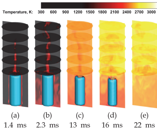
Fig. 4 Temporal evolution of temperature field and grain surface for single-grain burning.
