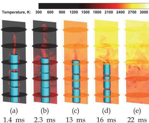
Fig. 8 Temporal evolution of temperature field and grain surface for three-grains burning.
