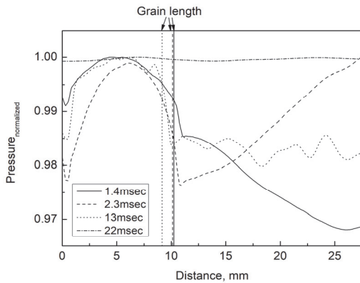
Fig. 7 Normalized pressure along the center line.
