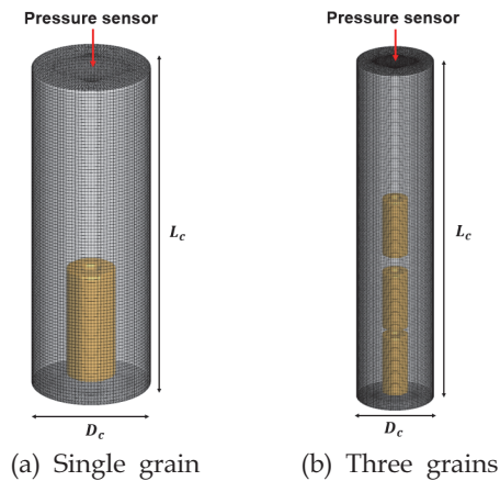
Fig. 2 Computational domain.
