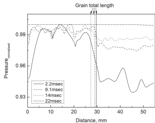
Fig. 10 Normalized pressure along the center line.
