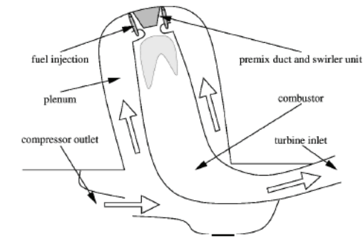
(a) Schematics of a real gas turbine combustor
