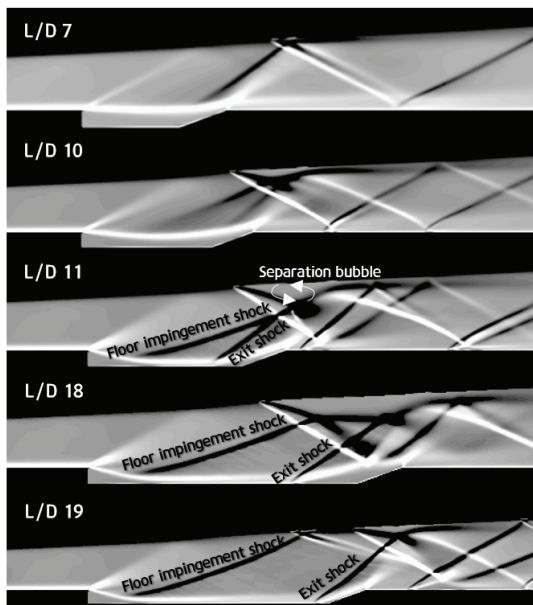
Fig. 11 Flow structures with cavity L/D (Depth = 4 mm, Ramp angle = 20°, Combustor height = 10 mm).
