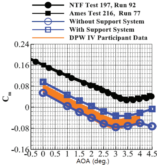
Fig. 2 Comparison of NTF and Ames 11-Ft TWT experimental data with USM3D CFD data and DPW IV CFD data for the without support system configuration, M_\infty = 0.85 , Re_c = 5 \times 10^{14} [14].
