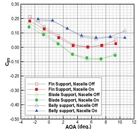
Fig. 14 Drag, Pitching moment coefficients vs alpha with Nacelle On/Off.
