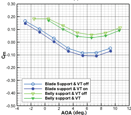
Fig. 13 Pitching moment coefficients vs alpha with VT on/off.
