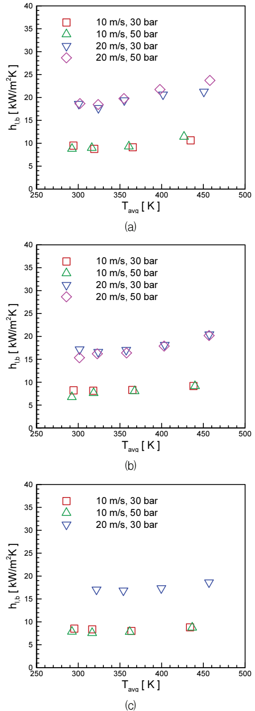
Fig. 7 Variation of convective heat transfer coefficient with average wall temperature at d_i = (a) 1.6 mm, (b) 2.0 mm, and (c) 2.4 mm.
