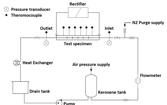
Fig. 3 Simplified electrical heat transfer test apparatus.
