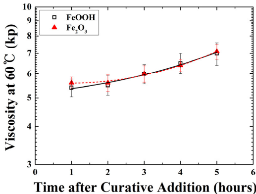
Fig. 1 Effect of burning rate catalyst on viscosity build-up.
