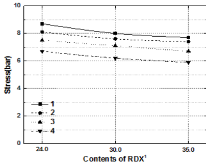
Fig. 3 Stress of propellants with different particle size of RDX.
