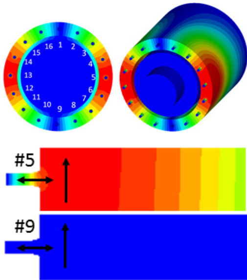
(b) Open boundary condition in nozzle
